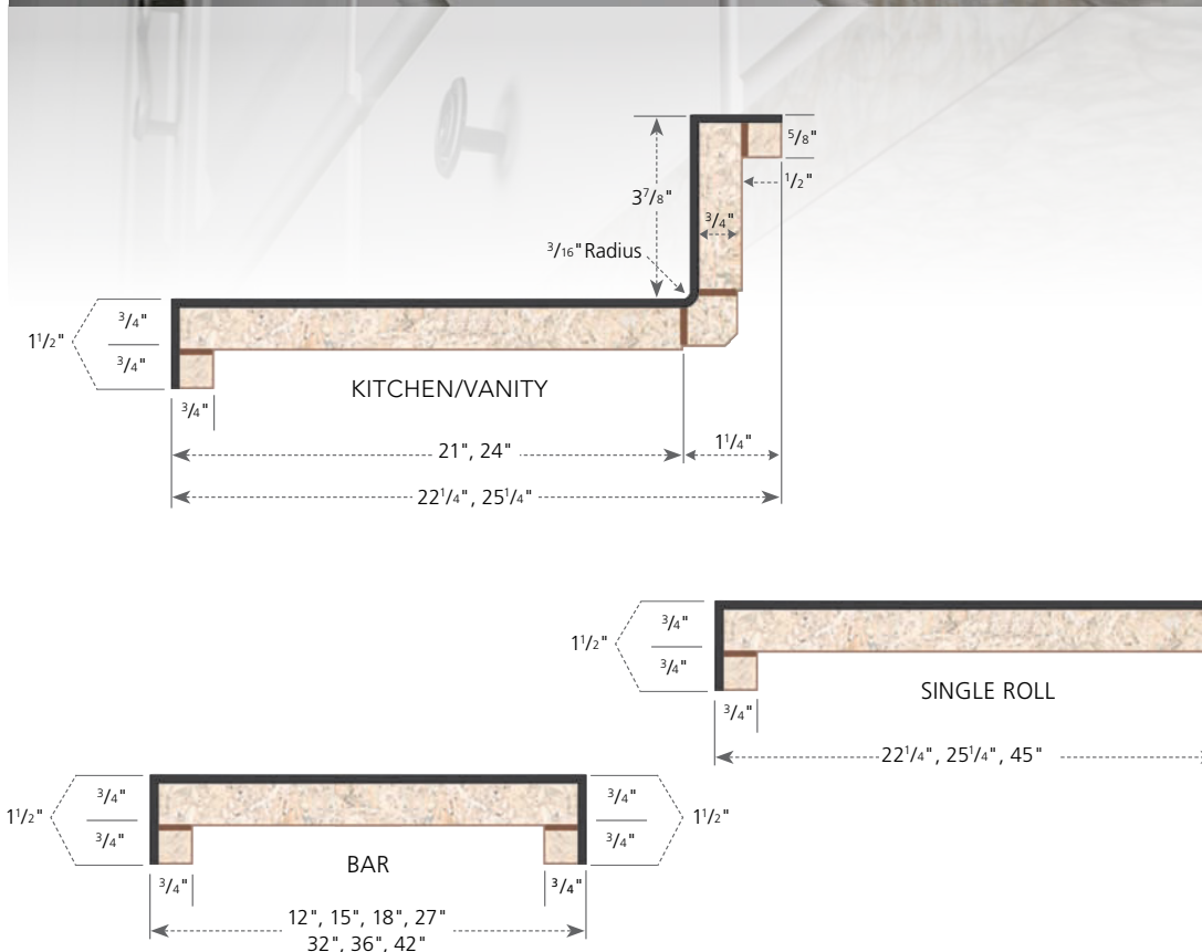
All measurements in inches. Drawings not to scale.
