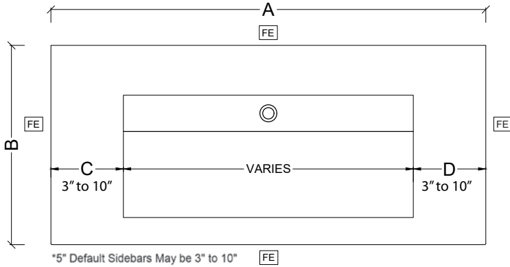
PLAN VIEW: TROUGH SINK
